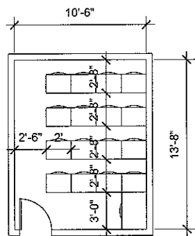
MINMUM STANDARD CLASSROOM LAYOUT (TO BE CONFIRMED)
